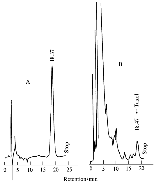
图 1 云南红豆杉培养细胞中紫杉醇的高效液相色谱图 Fig. 1 The HPLC chromatogram of taxol in the culture cells from Taxus yunnanensis
