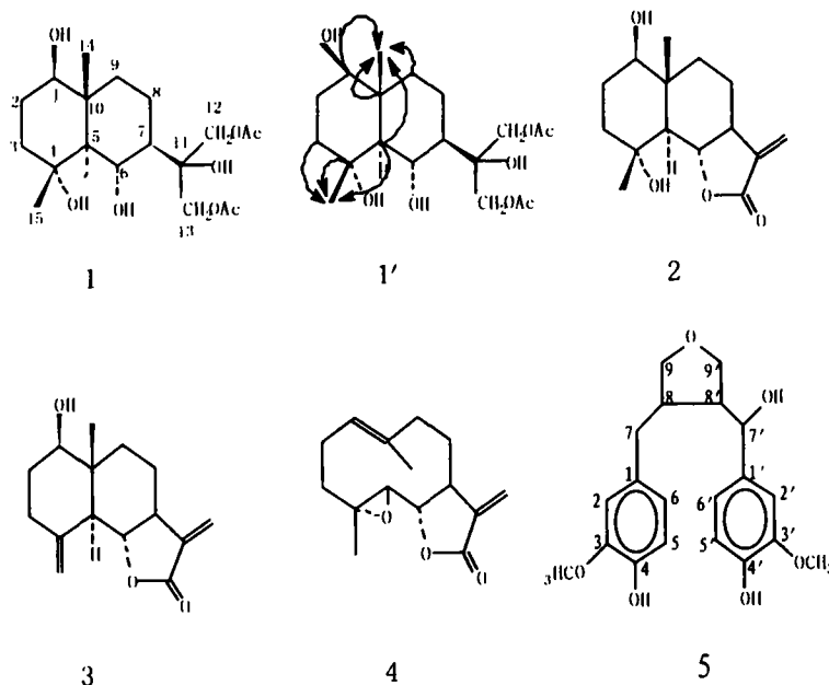
1': HMBC of compound 1 (C → H)
