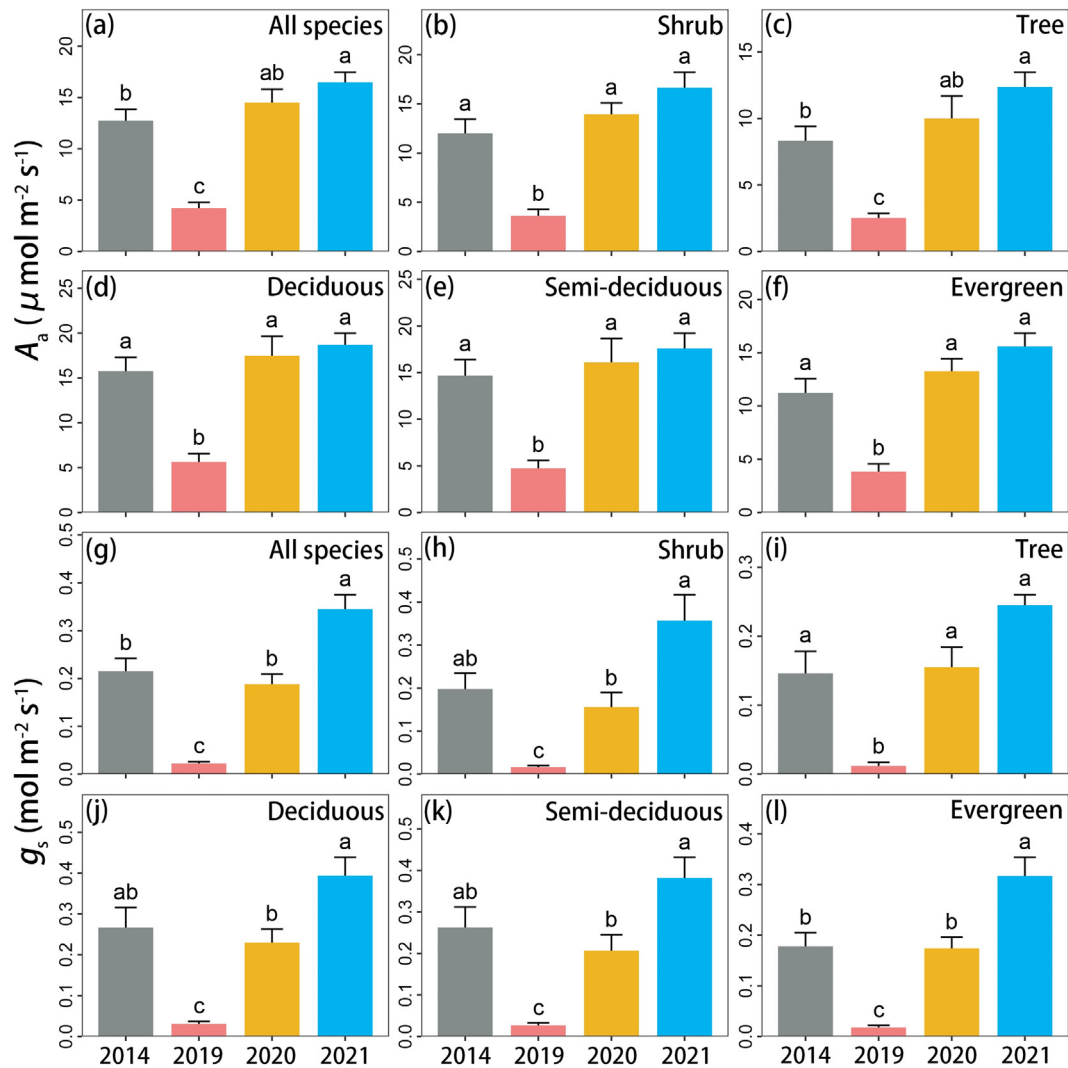
Fig. 4. Differences in mean trait values of (a–f) maximum photosynthetic rate per area ( A_a ) and (g–l) stomatal conductance ( g_s ) among four years (2014, 2019, 2020 and 2021) for all 16 species, different growth forms (shrub and tree) and leaf habits (deciduous, semi-deciduous and evergreen). Data on A_a and g_s of the 16 same species as in this study at the same site in 2014 (a regular year) were measured by Shu-Bin Zhang during the rainy season of 2014 (unpublished data). Error bars represent \pm 1 SE. Different letters on top of the error bars indicate significant difference in traits among years ( p < 0.05 ). One-way multivariate analysis of variance (ANOVA) was used to test the difference in traits, and the Bonferroni correction was used to adjust p values in multiple comparisons.
