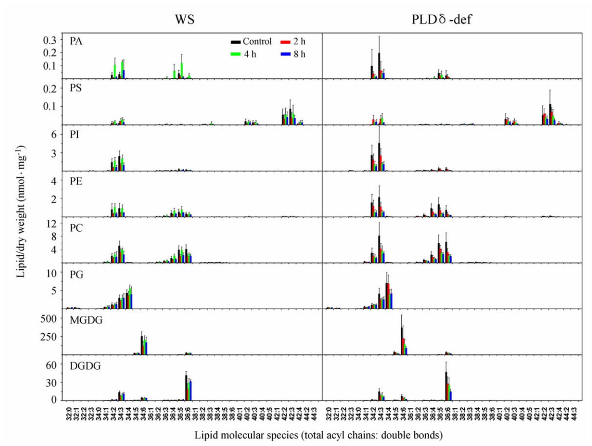
图 1 紫外辐射诱导的拟南芥膜脂分子变化。数值为平均值±标准差 (n=4 或 5) Fig. 1 Changes of lipid molecular species under UV-B irradiation in WS and PLD \delta -def plants. Values are means \pm S. D. (n=4 or 5)
