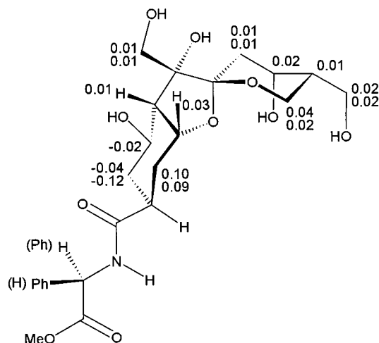
Figure 1. \Delta\delta(\text{S}-\text{R}) values (in ppm) for PGME amide derivatives of 1.
