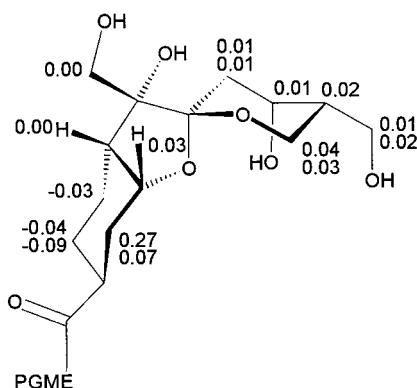
Figure 2. \Delta\delta(\text{S}-\text{R}) values (in ppm) for PGME amide derivatives of 2.
