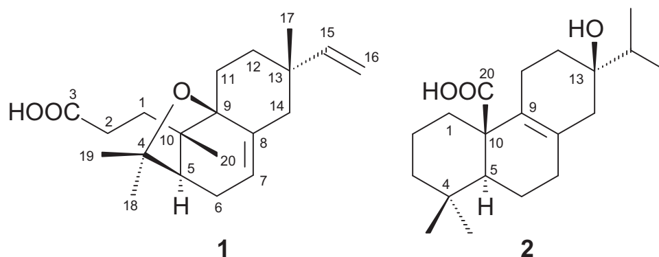
Fig. 1. Chemical structures of fladin A (1) and lophanic acid (2).
