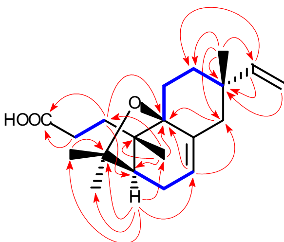
Fig. 2. Key COSY (— in blue) and HMBC (→ in red) correlations for 1.
