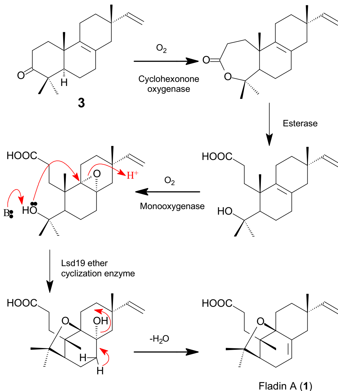
Fig. 4. Proposed biogenetic pathway of 1 .
