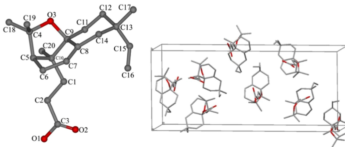
Fig. 3. X-ray crystallographic structure of 1.
