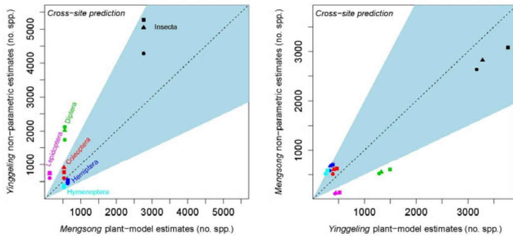
Figure 3 Cross-site predictions. Scatterplot of plant-model estimates versus non-parametric estimates of total OTU richness. Symbols as in Figure 2. Plant models from one landscape were used to predict non-parametric estimates in the other landscape. Shown here are the Mengsong wet-season results. Mengsong dry-season results are similar and shown in Figure S5. The shaded area encompasses a two-fold difference between the two estimates ( y = 0.5x to y = 2x ). The plant-model functions were Weibull for all taxa in Yinggeling and Mengsong, except for Lepidoptera in Mengsong, which was a linear function.
