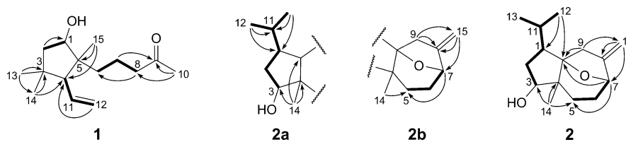
Fig. 2. Key HMBC (H \rightarrow C) and ^1\text{H},^1\text{H} -COSY ( \longleftrightarrow ) correlations of 1 and 2
