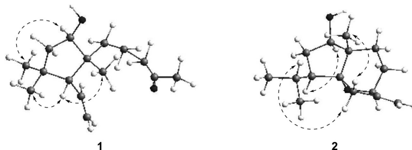
Fig. 3. ROESY (H \longleftrightarrow H) correlations of 1 and 2
