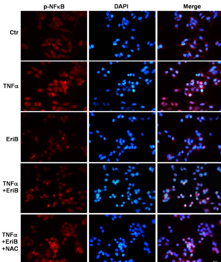
Fig. (S1). The intracellular translocation of p-NFκB (p65) was analyzed by immunofluorescence in CAPAN-2 cells. The experiment was repeated independently three times.
