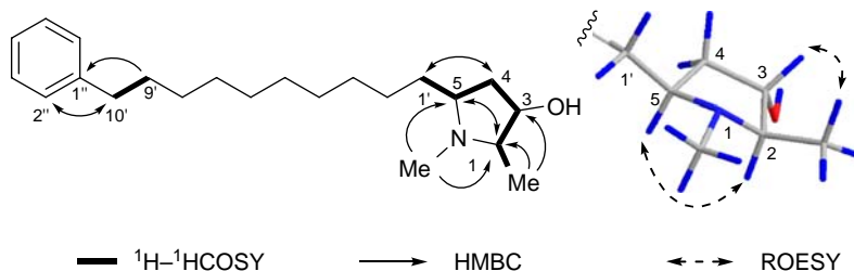
Figure 2. Key 2D NMR correlations of compound 1 .
