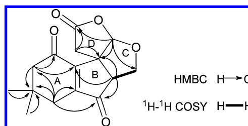
Figure 1. Key 2D NMR correlations of 1 .
