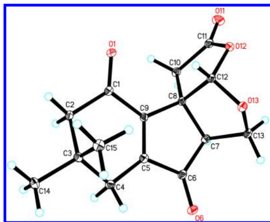
Figure 2. X-ray structure of 1 .
