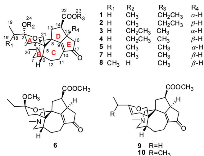
Figure 1. Structures of 1–10.
