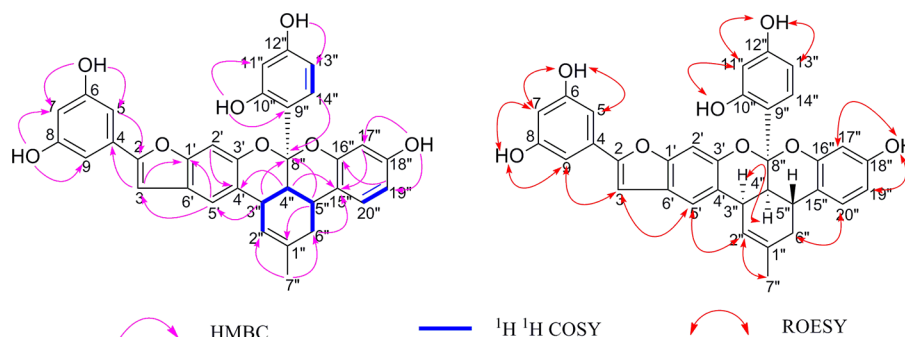
Figure 2. Selected 2D NMR correlations for isomulberrofuran G (2).
