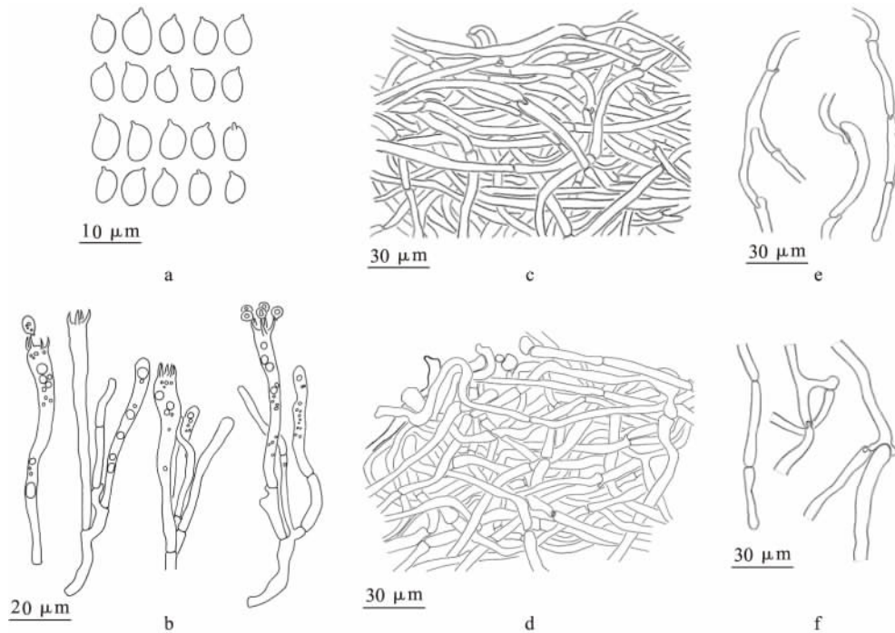
注: a. 担孢子; b. 担子; c. 鳞片菌丝; d. 该表皮非鳞片菌丝; e, f. 子实层偶见厚壁菌丝。 Note: a. spores; b. basidia; c. structure of squamules on pileus; d. pileipellis from an area not covered by squamules; e, f. few thick-walled hyphae from trama.
