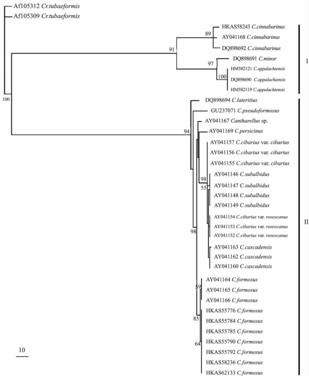
图 5 基于核糖体大亚基序列分析和最大简约法构建的最大简约树之一 Fig. 5 A phylogram of one of the most parsimonious trees by the analysis of the nuclear large subunit LSU
