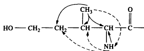
Scheme 1. Selected HMBC and NOESY for the amino acid residue (HOlle) in DMSO- d_6 .
